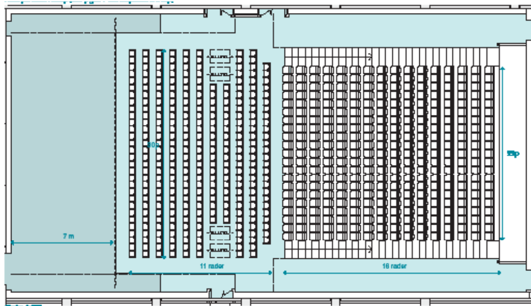
Cinema seating with 7m stage. Parquet about 660 people (270 chairs & 350 in the telescopic seating). Side balcony 130 people and upper balcony 163 people.
