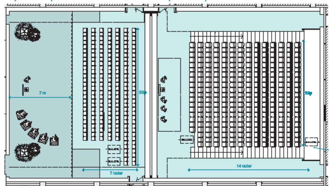
Cinema seating in two parts with partition. Stage side: 279 sqm for 200 people. Telescopic side: 336 sqm for 300 people
