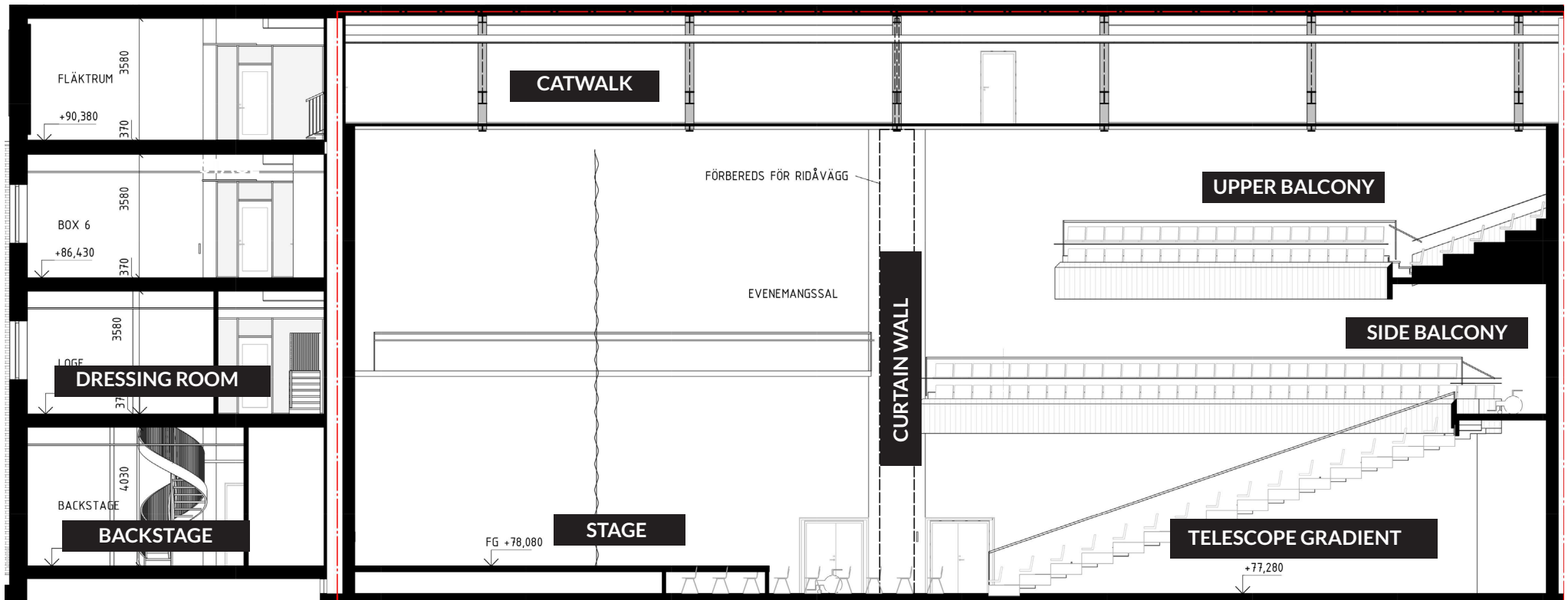
Section plan of the Event Hall, floor 1-4
